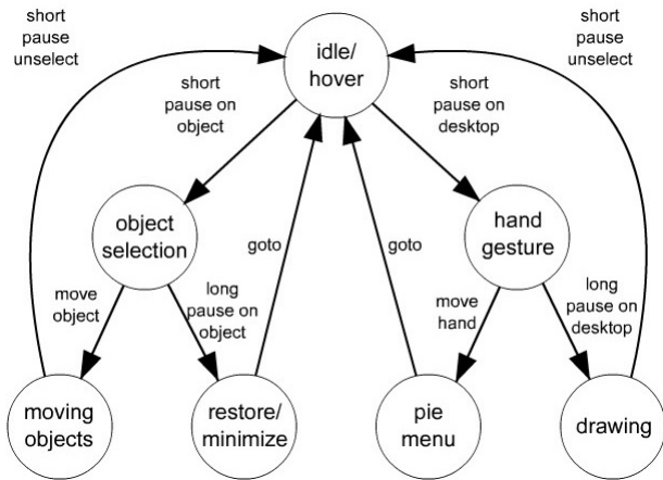
Figure 3. The WikiTUI state transition diagram. The circles represent the states and the edges are transitions.
